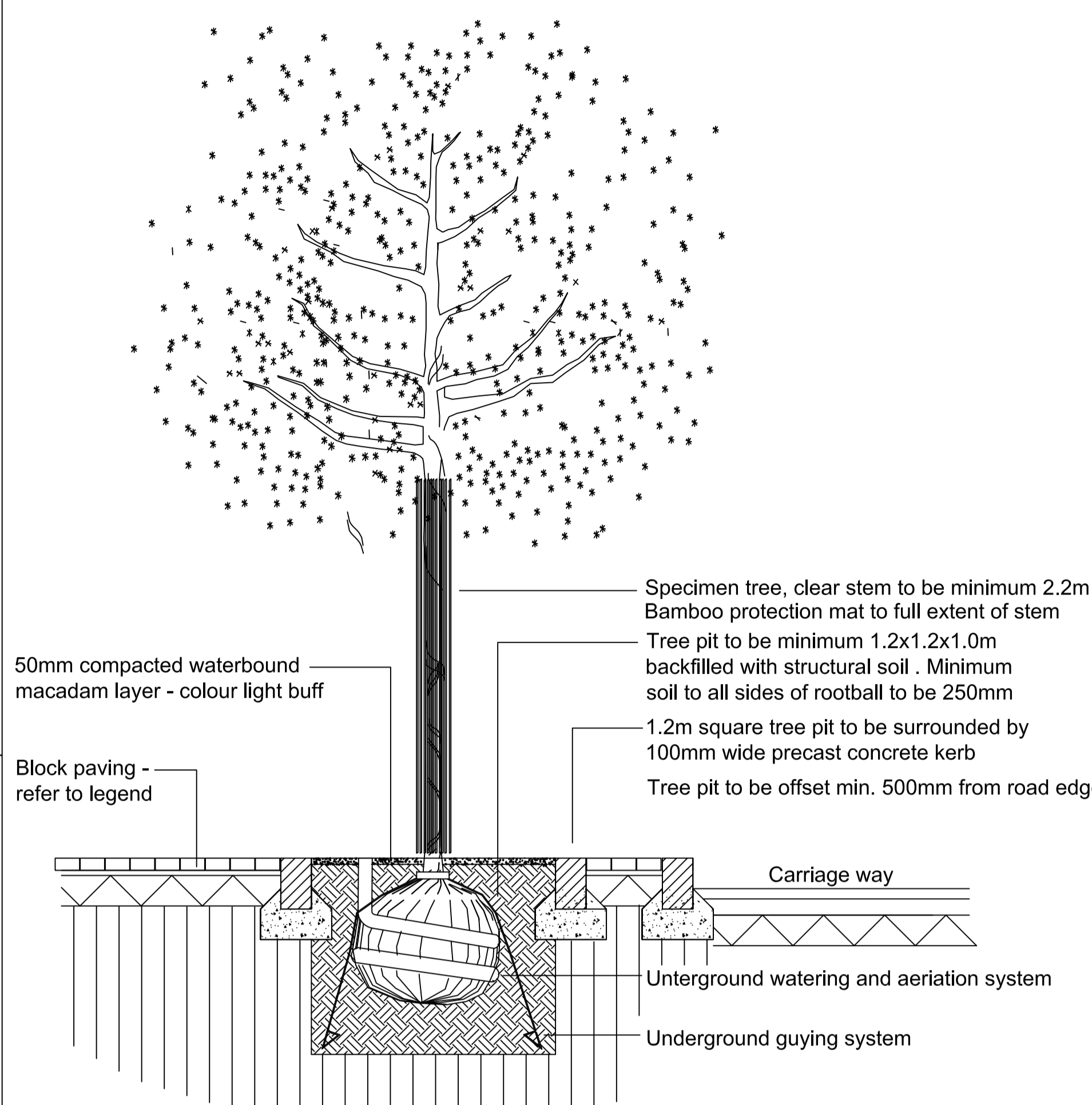
3 052 TYPICAL SECTION - TREE PIT AND ROAD FOOTPATH SCALE 1:25
