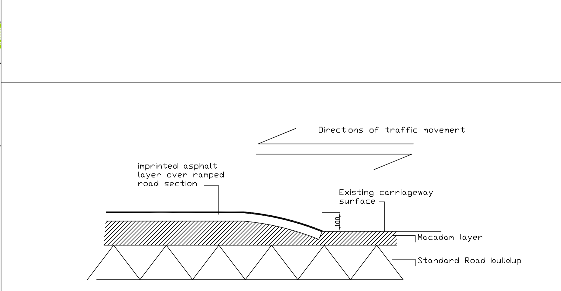
4 052 TYPICAL SECTIONS - RAMPED CARRIAGEWAY (INDICATIVE DETAIL) SCALE 1:15
